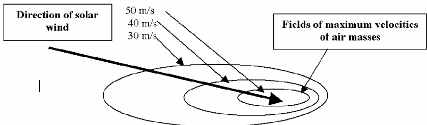
Figure 2. A representation of SW direction, and of the field of maximum velocity of air masses in the upper layers of the atmosphere
