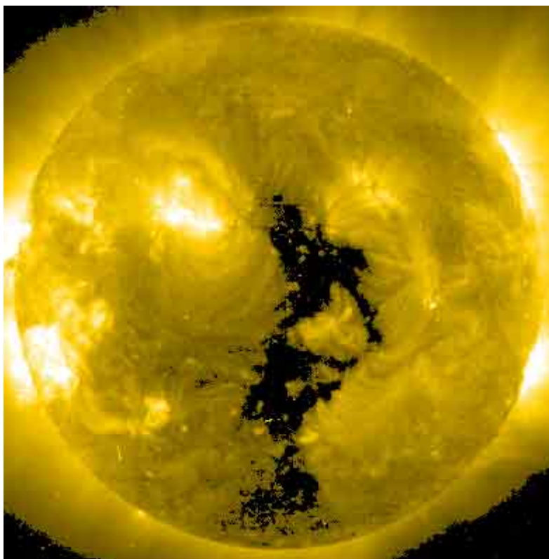
Figure 8. Sun photographed by a special electronic camera which uses extreme ultraviolet wavelengths, 284 Å*
