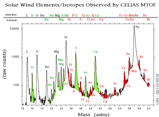
Figure 3. Example of chemical composition of SW
