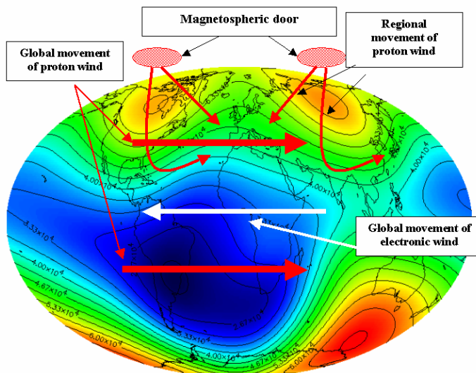
Figure 1. The map of most frequent positions of magnetospheric doors and paths of global and regional SWs
