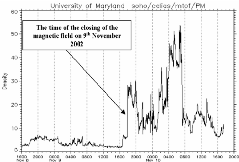
Figure 5. SW density diagram*
